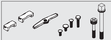
Nylon Bracket SHF-85-138 Spring SHF-85-107 Rivet SHF-85-160 Cross Head Screw SHF-85-131 Heald Frame Assembly Screw SHF-86-152
